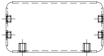
Front Panel
